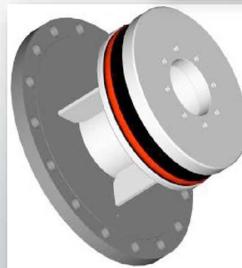
10" Flange Tester performing hydrotest on GRE pipe
